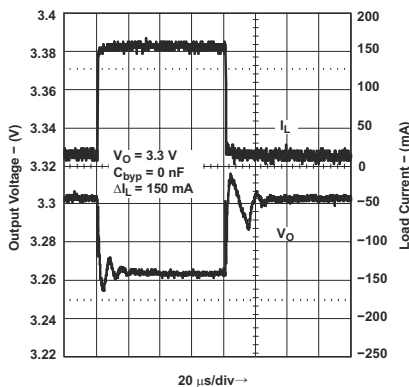
图 7-5. Load Transient Response for Legacy Chip
